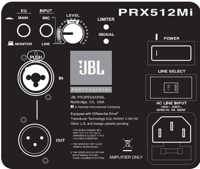
PRX512Mi Input Panel
