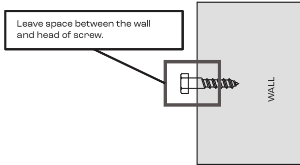
Wall anchor omitted for clarity.
