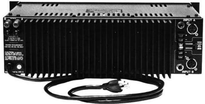
Back Panel Models 6230, 6260
