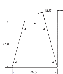
Top View all /64 & 95 models and PD5122
