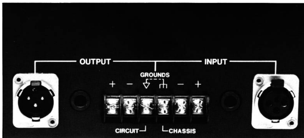
Rear Panel Connections
