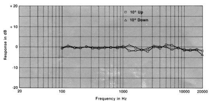
Vertical off-axis Response (normalized to on-axis) \pm 10^\circ Vertical
